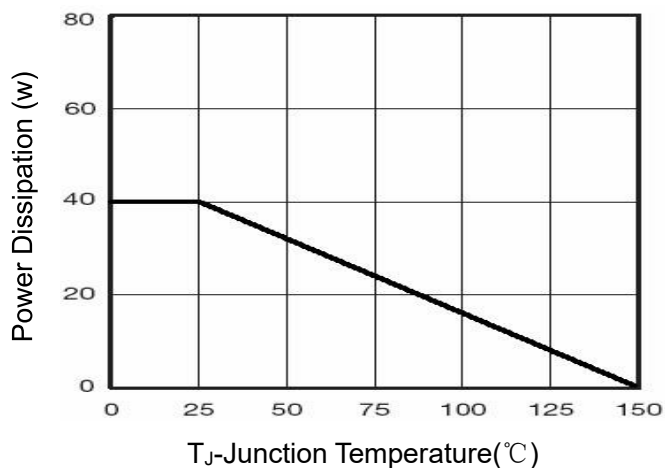
Figure 10 Power De-rating
