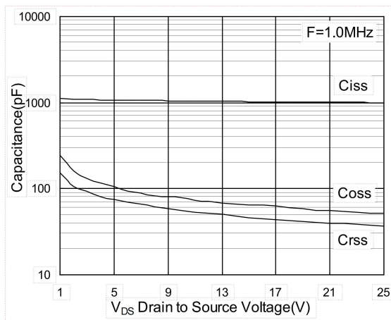
Fig.7 Capacitance
